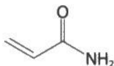
acrylamide
